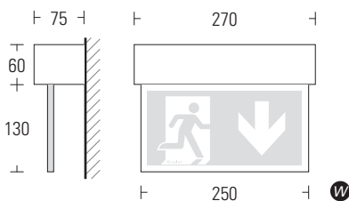
Wandmontage wall mounting
